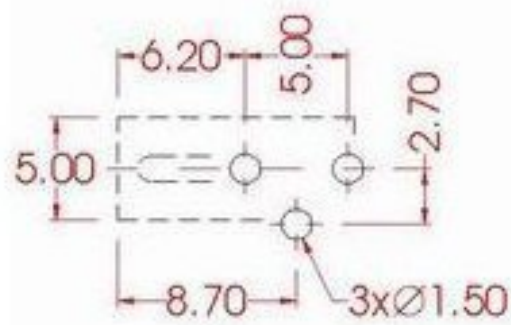
PIERCING PLAN
