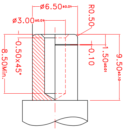
GAUGE PLUG
