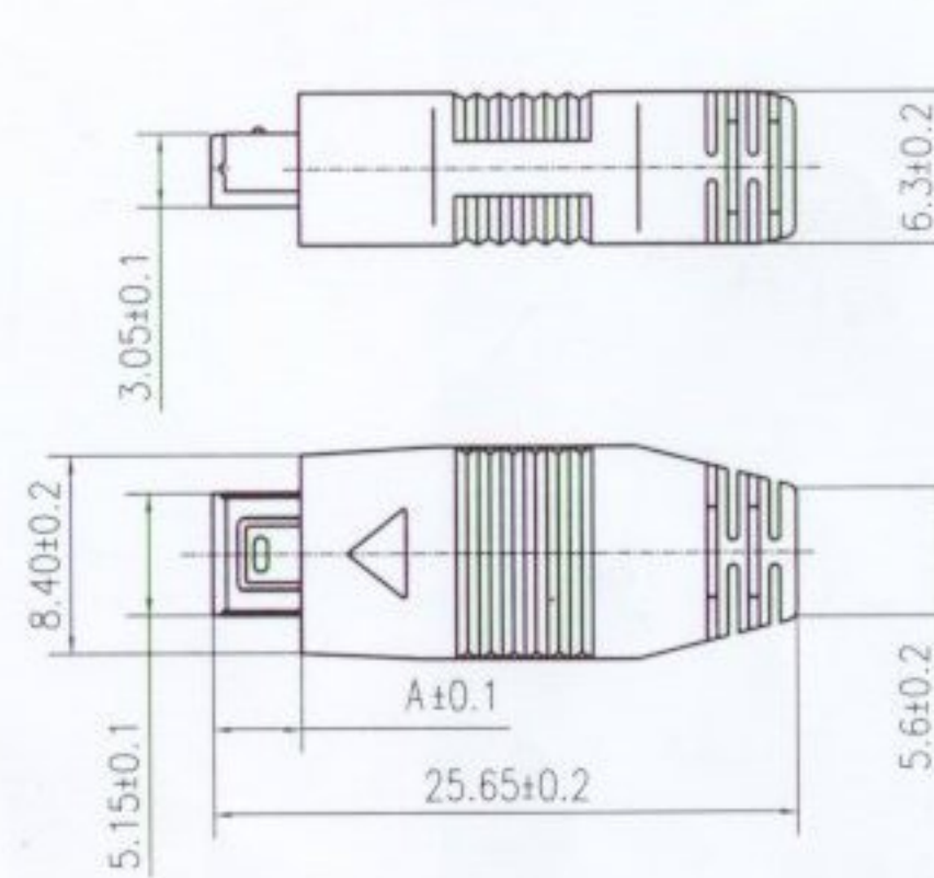
MIDDLE KEY
