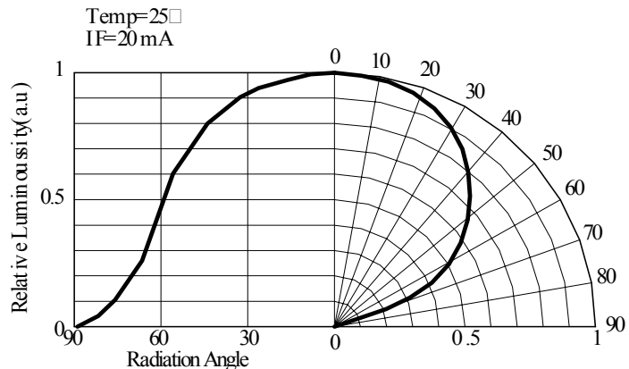
Radiation Diagram
