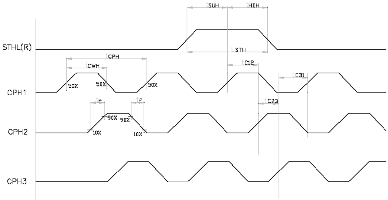
Fig.3-1 Sampling clock timing
