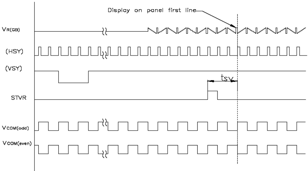
Fig.3-5(b) Vertical timing (from down to up)
