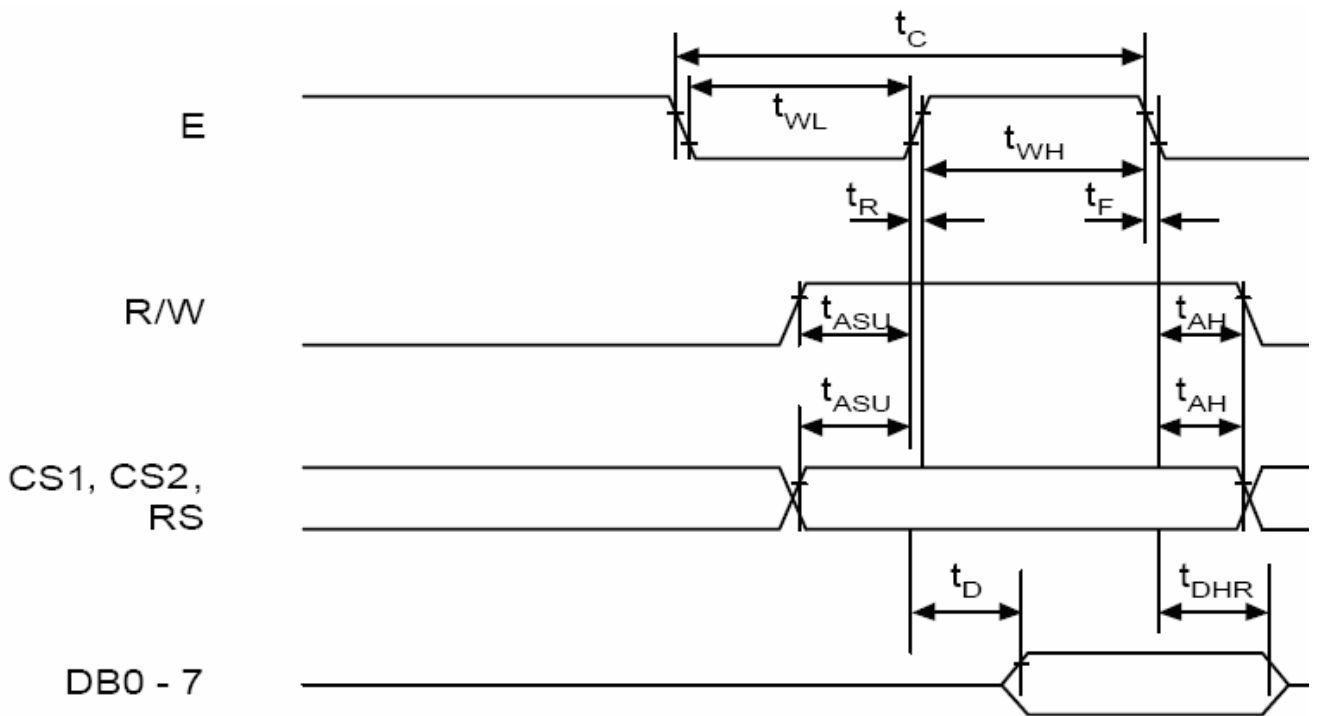
MPU Read Timing
