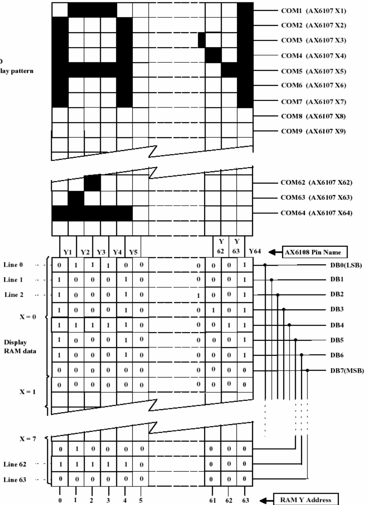
Fig 6 Relation between RAM Data and Display
