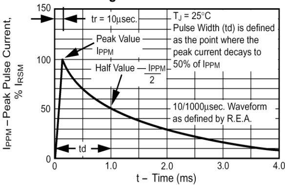
Fig. 3 – Pulse Waveform
