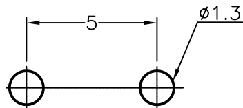
MOUNTING HOLES
